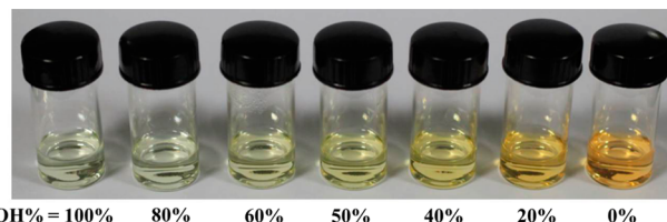
Figure 6. Photograph of (–)-1 ( 10^{-4} \text{ mol} \cdot \text{L}^{-1} ) in a mixed solution of MeOH and H 2 O in the ratios shown (under ambient light).
