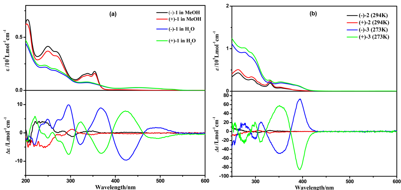
Figure 4. (a) UV–vis absorption and ECD spectra of (–)-1 and (+)-1 in MeOH and H 2 O at 5 \times 10^{-5} \text{ mol} \cdot \text{L}^{-1} . (b) UV–vis absorption and ECD spectra of (–)-2 and (+)-2 in dichloromethane at 5 \times 10^{-5} \text{ mol} \cdot \text{L}^{-1} (294 K) and (–)-3 and (+)-3 in dichloromethane at 2.5 \times 10^{-5} \text{ mol} \cdot \text{L}^{-1} (273 K).
